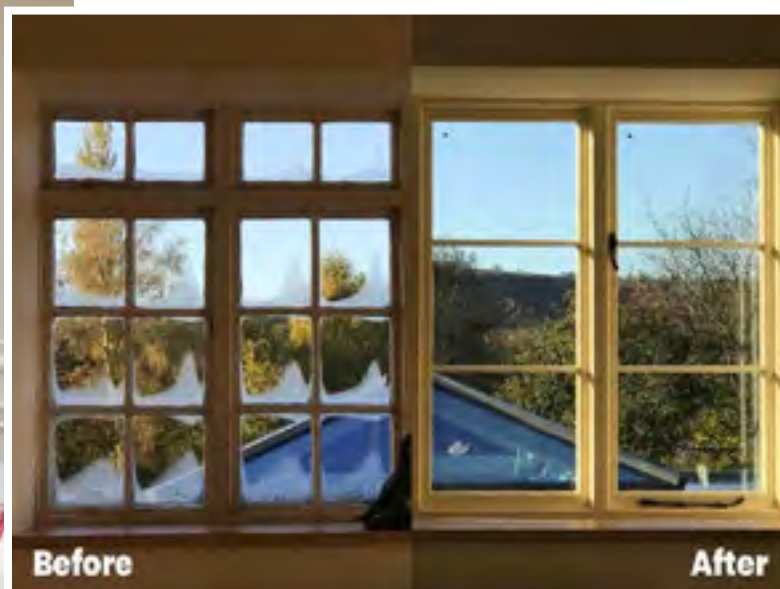
Internal condensation between single and vacuum glazing.
